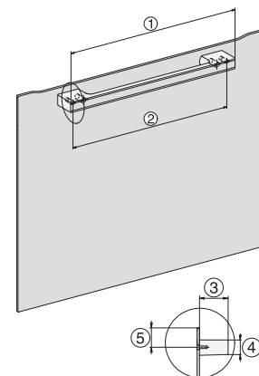
DG7x40, DGC7x4x, DGC7x6x, DG7635, DGM7x4x, DO7, H2860B/BP, H7240BM, H7x40BM, H7x4x8/BP, H7x6x8/BP, installation drawings
